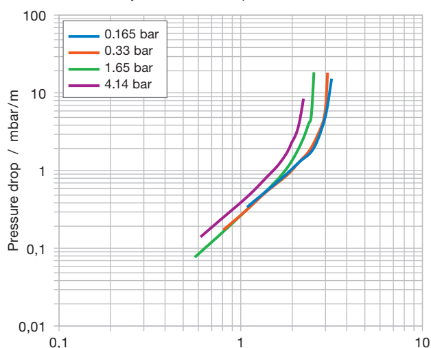
RMP N 250Y – Pressure drop Cyclohexane/n-Heptane, Total Reflux
