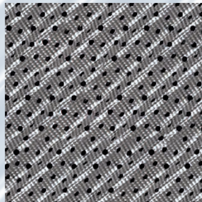
RMP N250Y structured packing with perforated and textured surface
